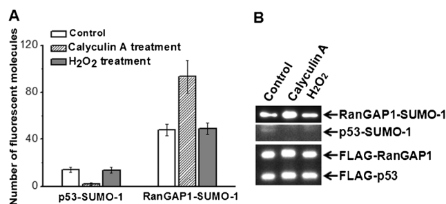
Figure 4. Simultaneous SUMOylation measurement under different physiological conditions. A) Number of fluorescent molecules measured in response to phosphatase inhibition (Calyculin A) or oxidative stress (H 2 O 2 ). Cells without any treatment were used as a control. Error bars show the standard deviation from three experiments. B) Measurement of SUMOylated RanGAP1 (upper panel), SUMOylated p53 (middle panel), and the total protein (lower panel) in (A) by western-blot assay.
